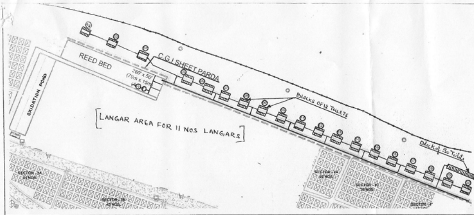
SITE PLAN OF STP AT BALTAL
